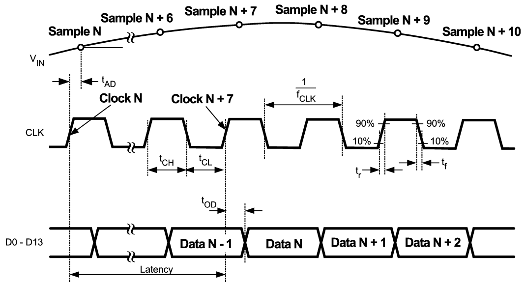
Output Timing
